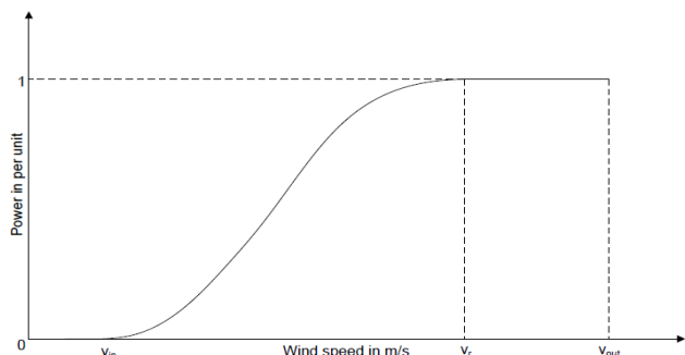
Fig. 1 A typical power- wind speed curve
