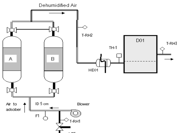
Fig. 3 Schematic overview of the experimental equipment. Internal diameter of columns A and B is 0.12 m, diameter of piping is 0.05 m, tray dryer size 0.40x0.25x0.60 m (Djaeni et al. 2012a).
