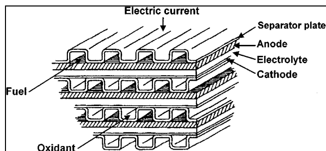
Fig. 3 Schematic representation of an interconnector (Samson Nesaraj, 2010) in SOFC
