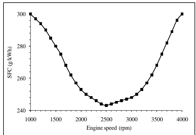
Fig. 10 Variation of SFC with engine speed, adapted from Kipor Power (2010)
