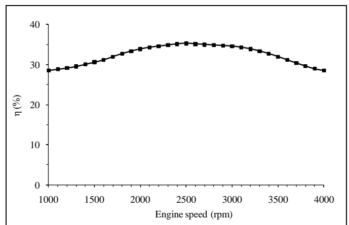
Fig. 11 Variation of efficiency with engine speed, adapted from Kipor Power (2010)
