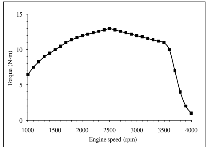
Fig. 9 Variation of torque with engine speed, adapted from Kipor Power (2010)
