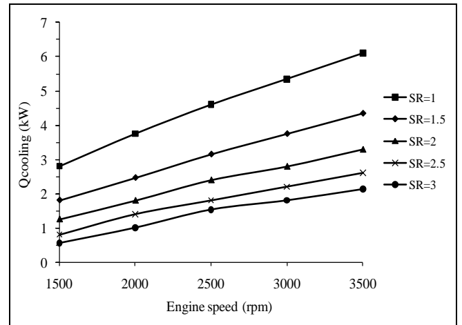
Fig. 14 Cooling capacity of the compact module system as a function of engine speed and SR
