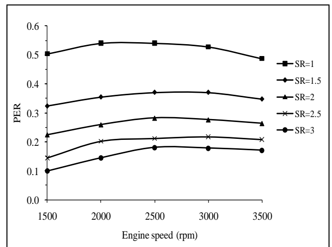
Fig. 15 Performance of the compact module system as a function of engine speed and SR
