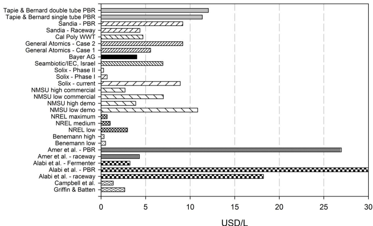
Fig. 5 Cost estimates for microalgae to oil production (adapted from USDoE, 2009; Pienkos, 2008)
