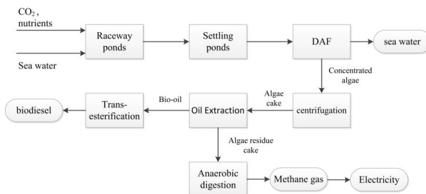
Fig. 1 Process diagram for production of biodiesel from microalgae used by Campbell et al. (2008, 2011)
