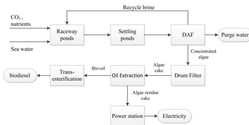
Fig. 2 Process diagram for production of biodiesel from microalgae used by Griffin & Batten (2009)
