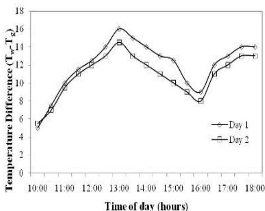
Fig. 5 Variation of temperature difference between glass and water temperature with effect of PCM
