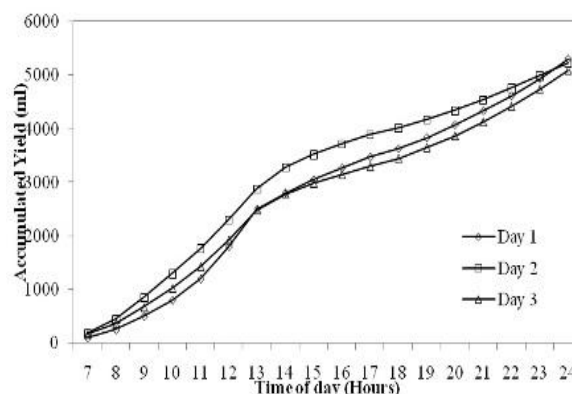
Fig. 9 Accumulated fresh water production with PCM
