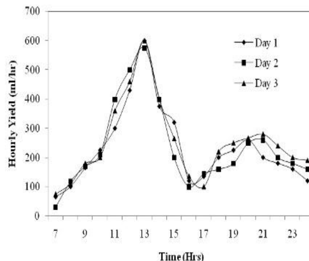
Fig. 3 Hourly variation of distillate output on different test days with PCM
