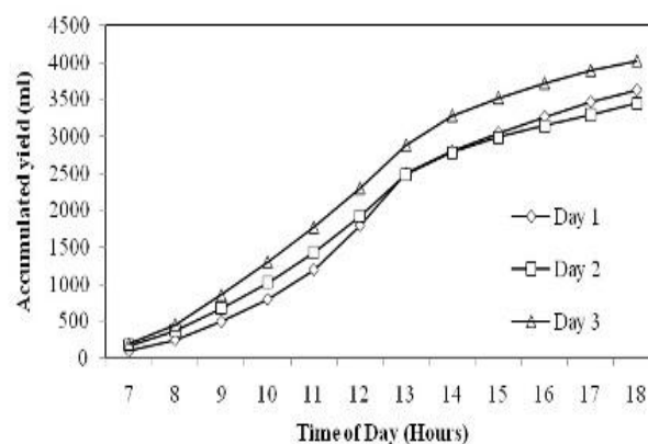
Fig. 8 Accumulated fresh water production without PCM
