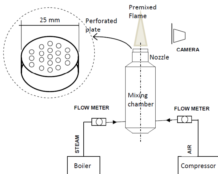
Fig. 1 Experimental apparatus
