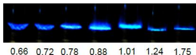
Fig. 6 Flame shapes of coconut oil without glycerol isolated from surrounding ambient air
