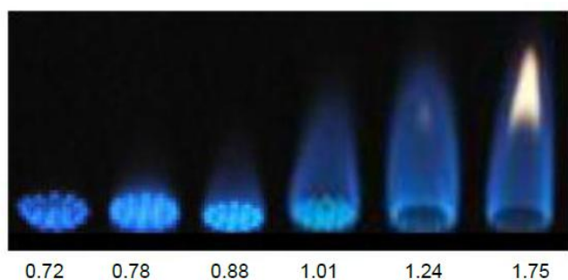
Fig. 5 Flame shape of coconut oil without glycerol
