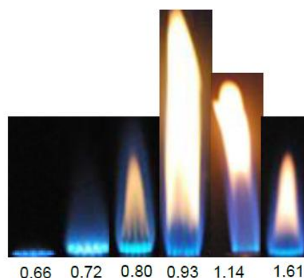
Fig. 2 Flame structure of coconut oil with glycerol
