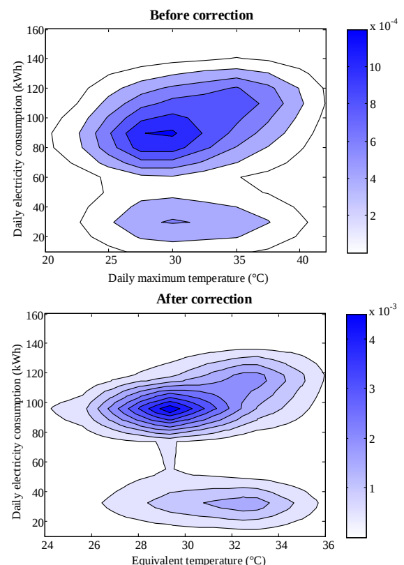
Fig. 4 Comparison of electricity-temperature kernel density estimation results before and after thermal inertia correction
