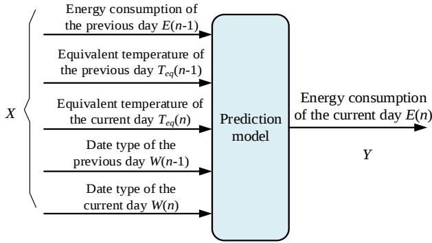
Fig. 2 Overall Structure of the prediction model
