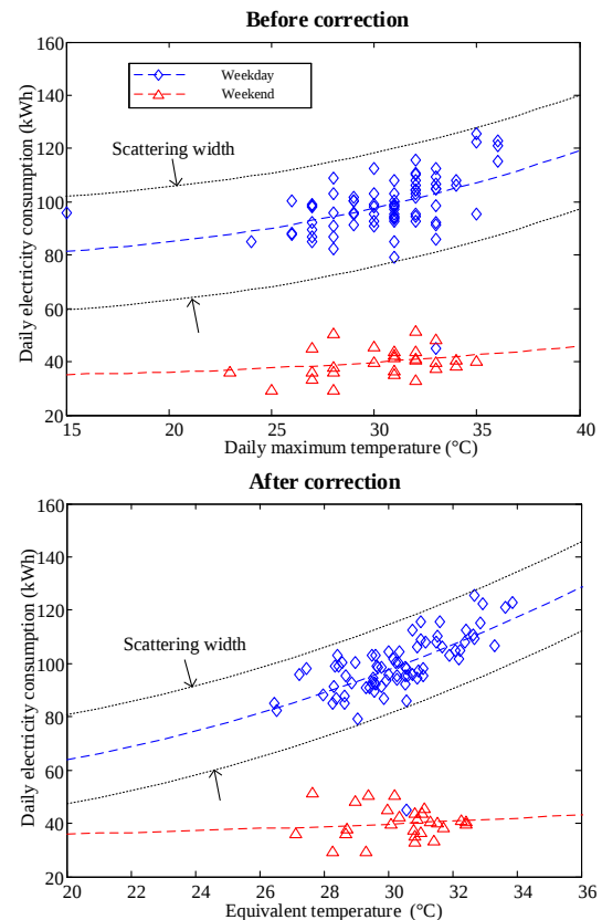
Fig. 3 Comparison of electricity-temperature scatter plot before and after thermal inertia correction
