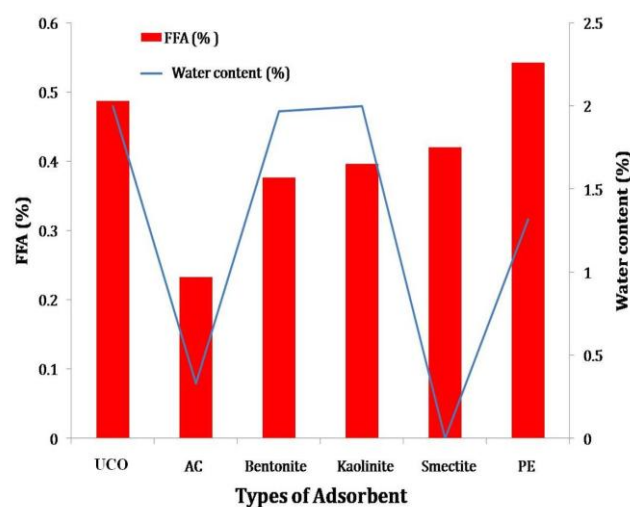
Fig. 1 The FFAs and water content for used-cooking oil after adsorption process by using various adsorbent compared with the oil without pre-treatment process
