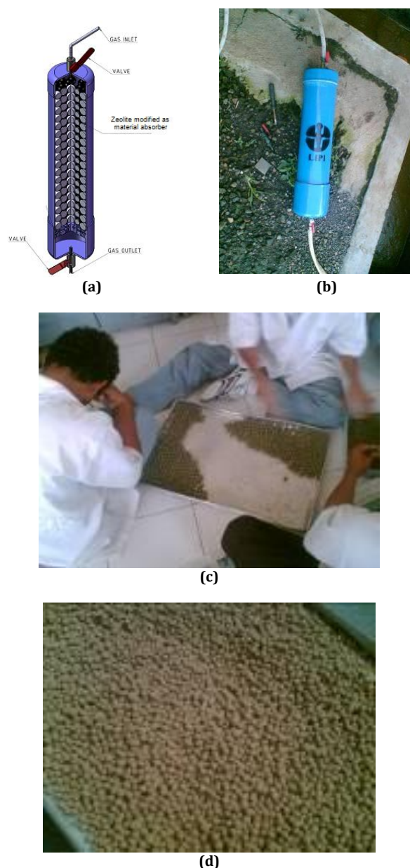
Fig. 1 The biogas filter : (a) Diagram; (b) Cylindrical tube; (c) Zeolite modification process; (d) Modified natural zeolite
