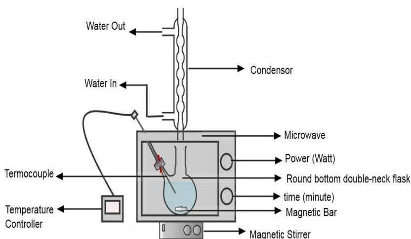
Fig. 1 Experimental set-up of the microwave-assisted biodiesel reactor unit.
