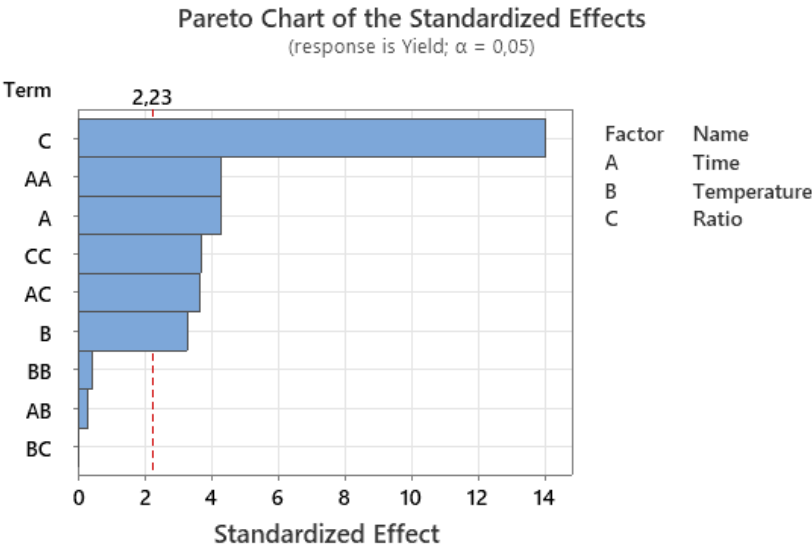
Fig. 5 Pareto chart of standardized effects for FABE yield optimization.
