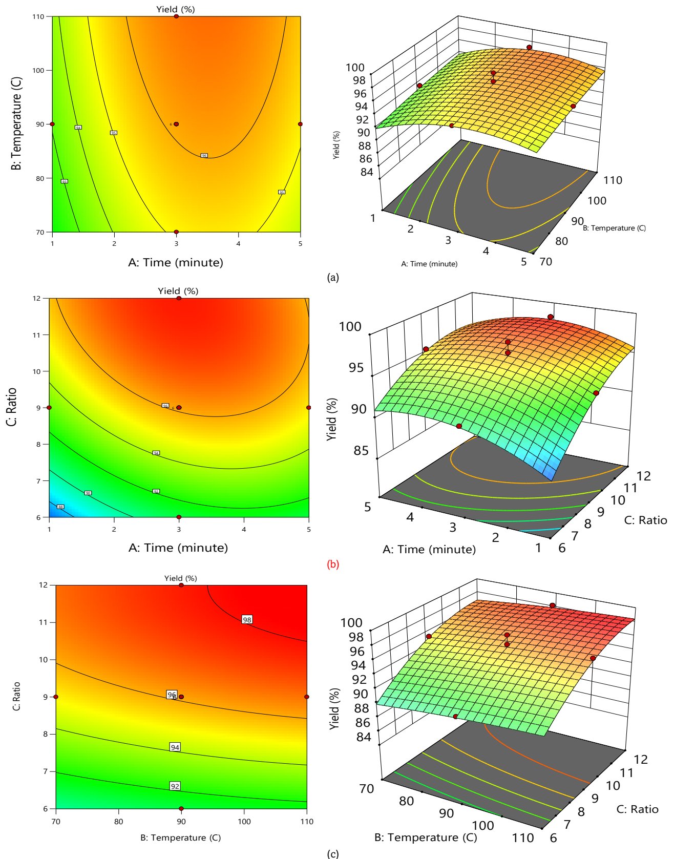
Fig 6. Contour and three-dimensional response surface plots for FABA yield as a function of: (a) reaction time and temperature; (b) reaction time and reactant molar ratio; and (c) temperature and reactant molar ratio.
