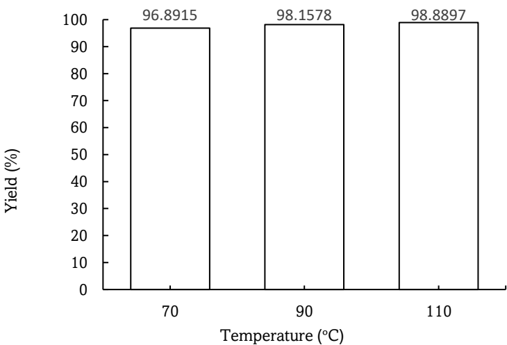
Fig. 2 Effect of reaction temperature on biodiesel yield.
