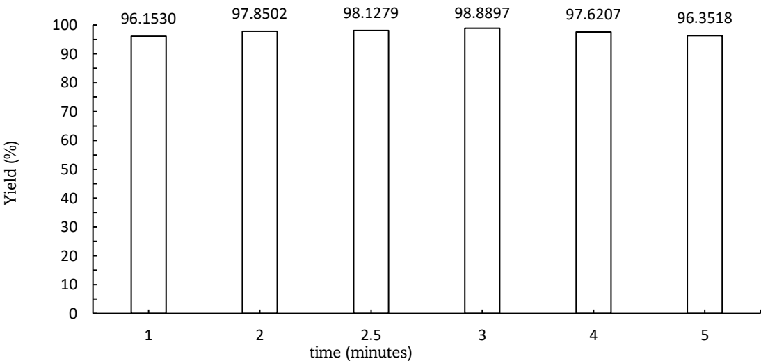
Fig. 3 Effect of reaction time on biodiesel yield.
