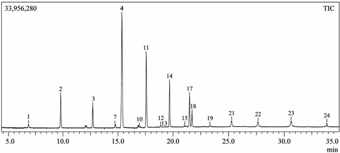
Fig. 9 GC-MS result of butyl ester obtained
