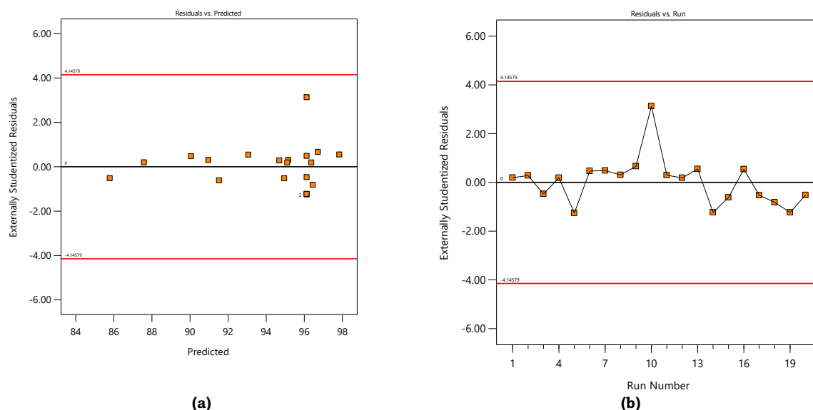
Fig. 8 Residual diagnostic plots for the FCCD regression model of Fabe yield: (a) residuals versus predicted values and (b) residuals versus experimental run order.
