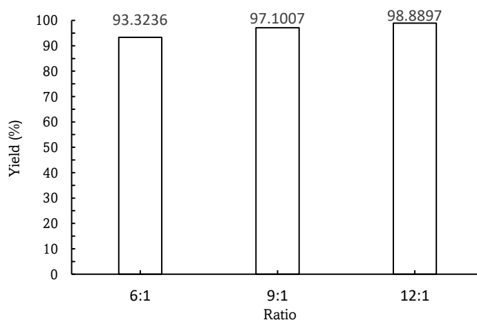
Fig. 4 Effect of butanol-to-oil molar ratio on biodiesel yield.
