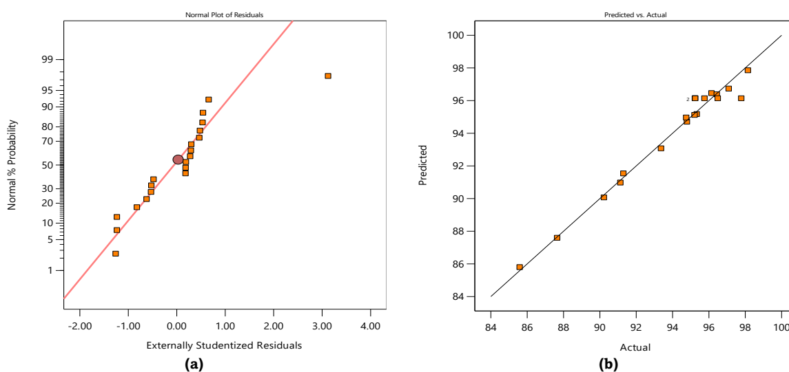
Fig. 7 Diagnostic plots for the FCCD regression model of FAFE yield: (a) normal probability plot of residuals and (b) predicted versus actual values
